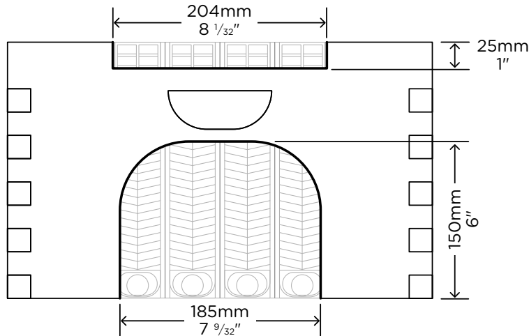
10 FRAME LANGSTROTH SUPER Cutouts required to fit 4 Flow™ frames
