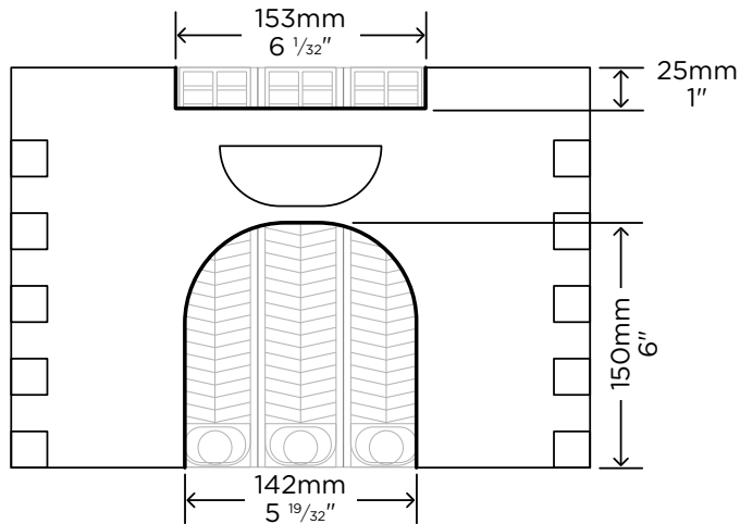
8 FRAME LANGSTROTH SUPER Cutouts required to fit 3 Flow™ frames
