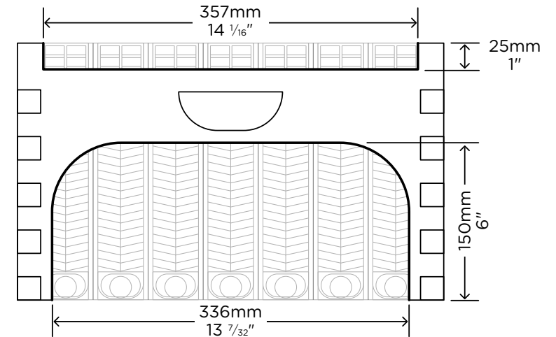
10 FRAME LANGSTROTH SUPER Cutouts required to fit 7 Flow™ frames
