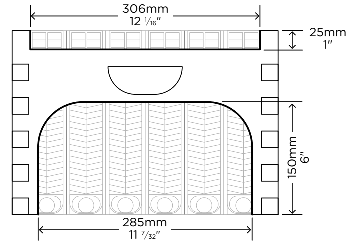
8 FRAME LANGSTROTH SUPER Cutouts required to fit 6 Flow™ frames
