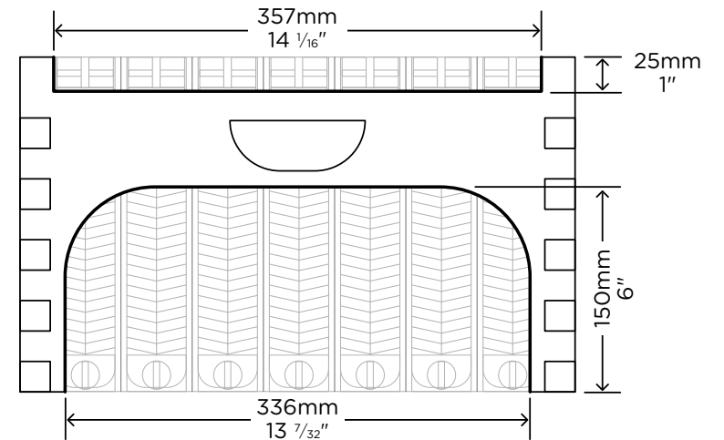
Cutouts required to fit 7 Flow Frames
