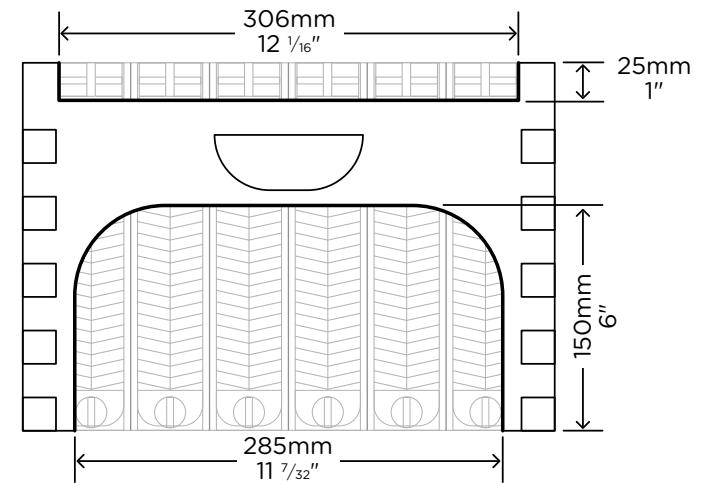
Cutouts required to fit 6 Flow Frames
