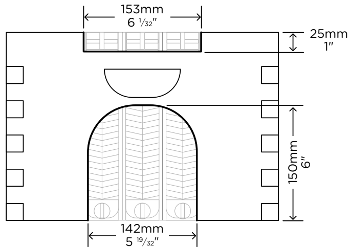
Cutouts required to fit 3 Flow Frames
