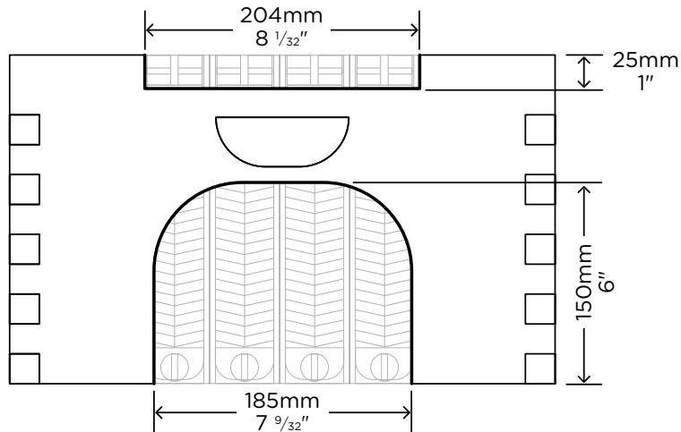
Cutouts required to fit 4 Flow Frames
